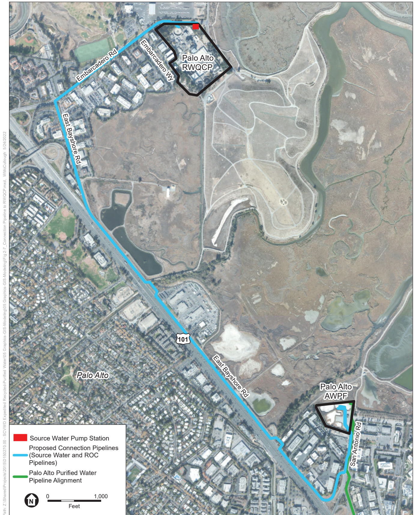
Figure 2-7 Connection Pipelines between the Palo Alto Advanced Water Purification Facility and the Palo Alto Regional Water Quality Control Plant
